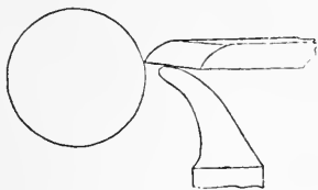
FIG. 292. INCORRECT POSITION OF GOUGE IN ROUGHING OFF.
